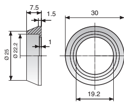
Protective collar 804757
